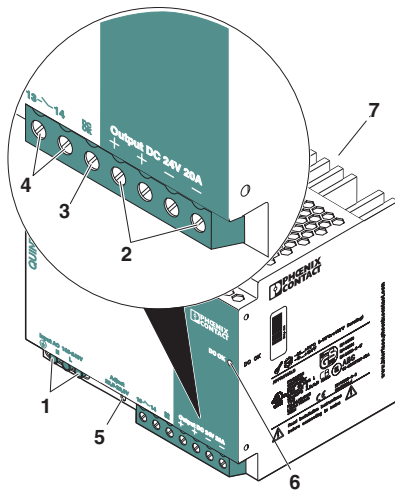
Figure 1 Operating elements
