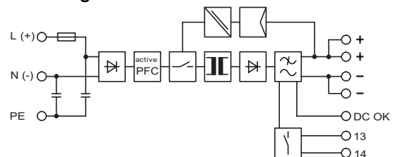
Figure 2 Block diagram
