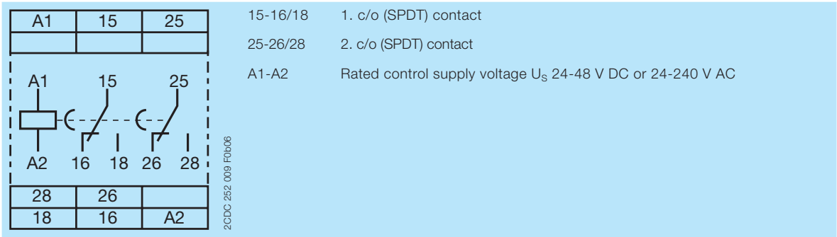
Connection diagram
