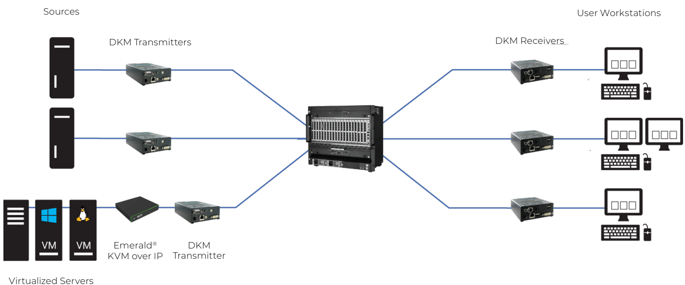
Fig 1.: DKM matrix switching setup connects multiple source computers and user workstations
