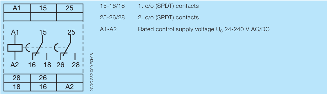
Connection diagram
