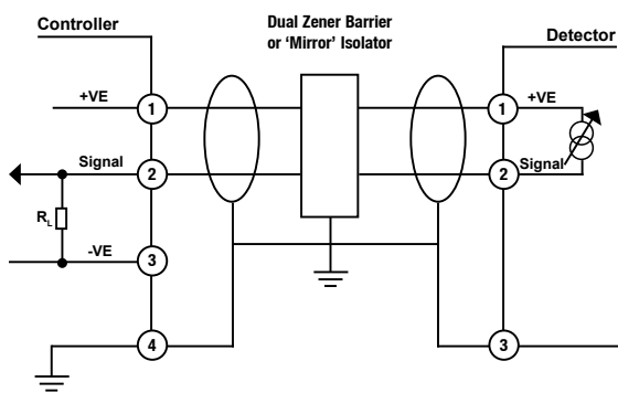
Dual Barrier Schematic
