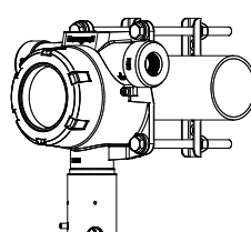
Pipe Mounting
