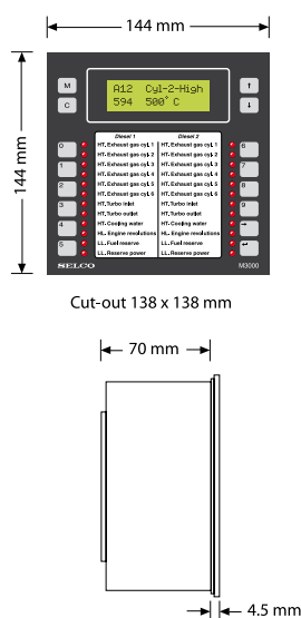
Fig. 9. Dimensions.
