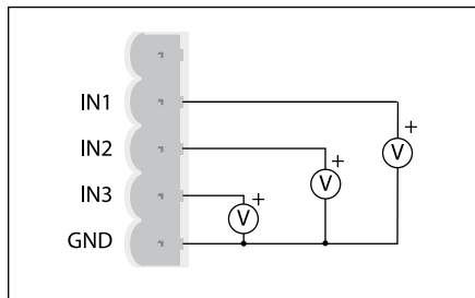
Fig. 1. 3 x Voltage inputs. It is possible to connect to three sensors with voltage output to each input group. The output from each sensor must be connected between an input terminal and the negative reference terminal.
