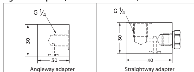
Figure 3: Adapters (stainless steel version)
