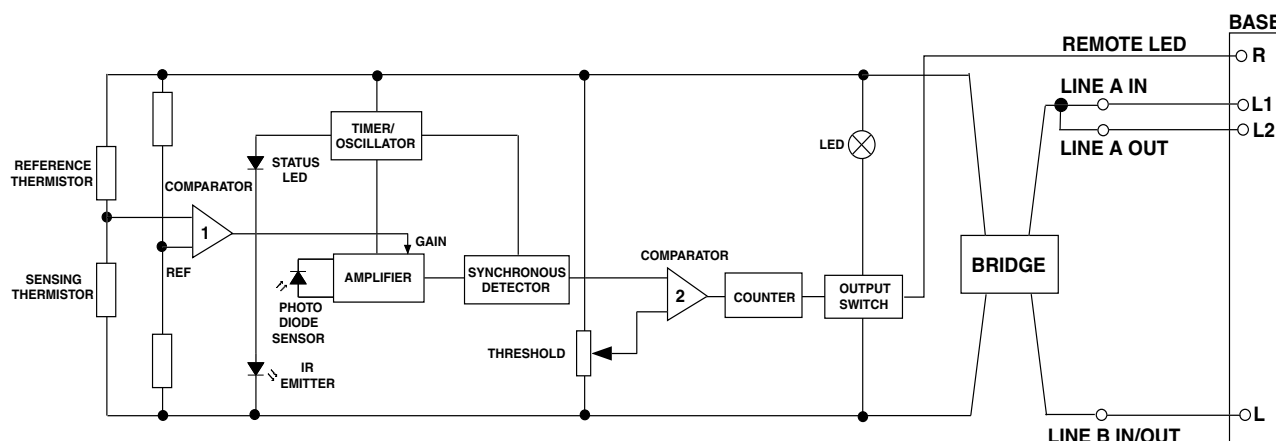
Fig. 4 Block Schematic of Detector
