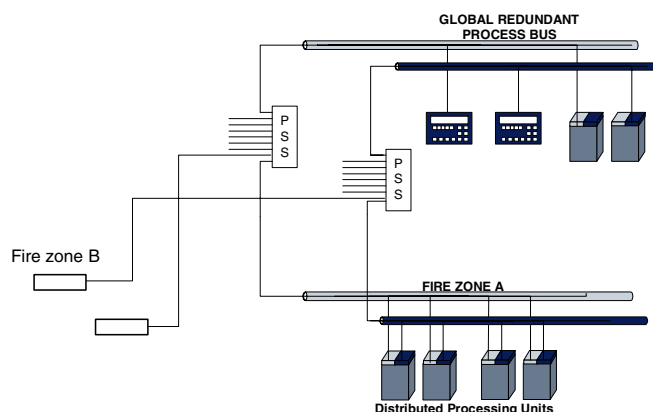
Principle for fire zone protection.
